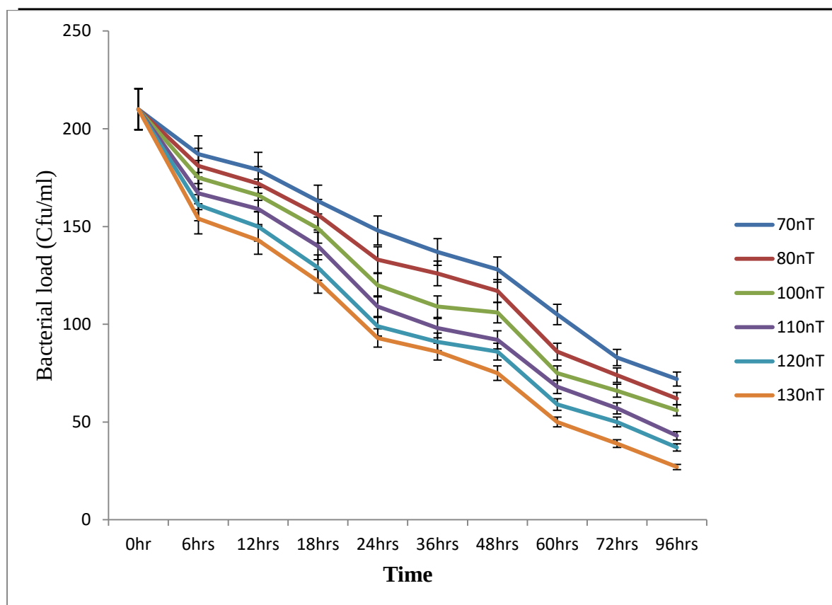
Figure 2: Effect of EMF at different intensities and time intervals on bacterial loads of brewery effluent
