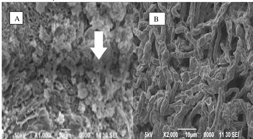
Figure 10: SEM micrographs of Fusarium equiseti KR706303 loaded with copper (A), and unloaded with metal (B). Arrow indicate the metal ions.
