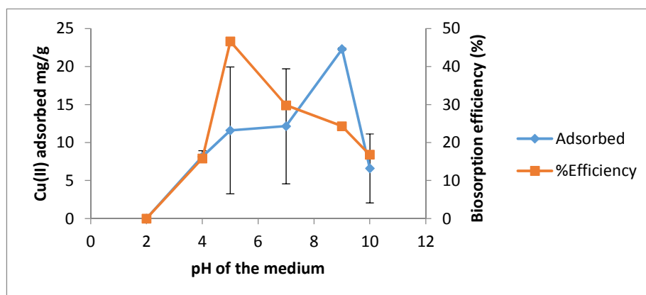
Figure 3: Copper (II) biosorption ( \text{mg g}^{-1} d.wt) and biosorption efficiency by Fusarium equiseti KR706303 at different pH values. Amount of dried biomass: 0.04\text{g} ; initial metal concentration (Ci): 50\text{ mg L}^{-1} ; suspension
