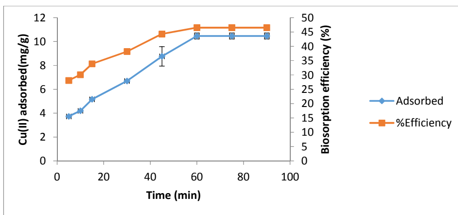
Figure 8: Copper (II) biosorption ( \text{mg g}^{-1} d.wt) and biosorption efficiency by Fusarium equiseti KR706303 at different time intervals. Amount of dried biomass: 0.04 g; initial metal concentration ( C_i ): 50 \text{ mg L}^{-1} ; suspension volume: 20 mL; temperature: 30°C; pH: 9; agitation speed: 150 rpm. The data are the mean values of 3 replicates, and the bars indicate the standard deviation of the mean.
