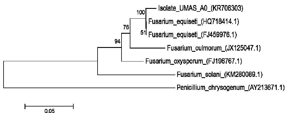
Figure. 2: Neighbour-joining tree from ITS sequences showing the relationship between the isolated indigenous fungus UMAS A0 and other closely related Fusarium species retrieved from the GenBank(accession number). Bootstrap values >70% (1000 replicates) are shown on the branches. Bar = 5 nucleotide substitution per 100 nucleotides.
