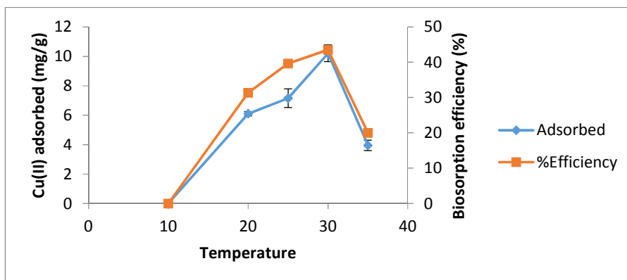
Figure 4: Copper (II) biosorption ( \text{mg g}^{-1} d.wt) and biosorption efficiency by Fusarium equiseti KR706303 at different temperatures. Amount of dried biomass: 0.04 g; initial metal concentration ( C_i ): 50 \text{mg L}^{-1} ; suspension volume: 20 mL; pH: 9; agitation speed: 150 rpm. The data are the mean values of 3 replicates, and the bars indicate the standard deviation of the mean.
