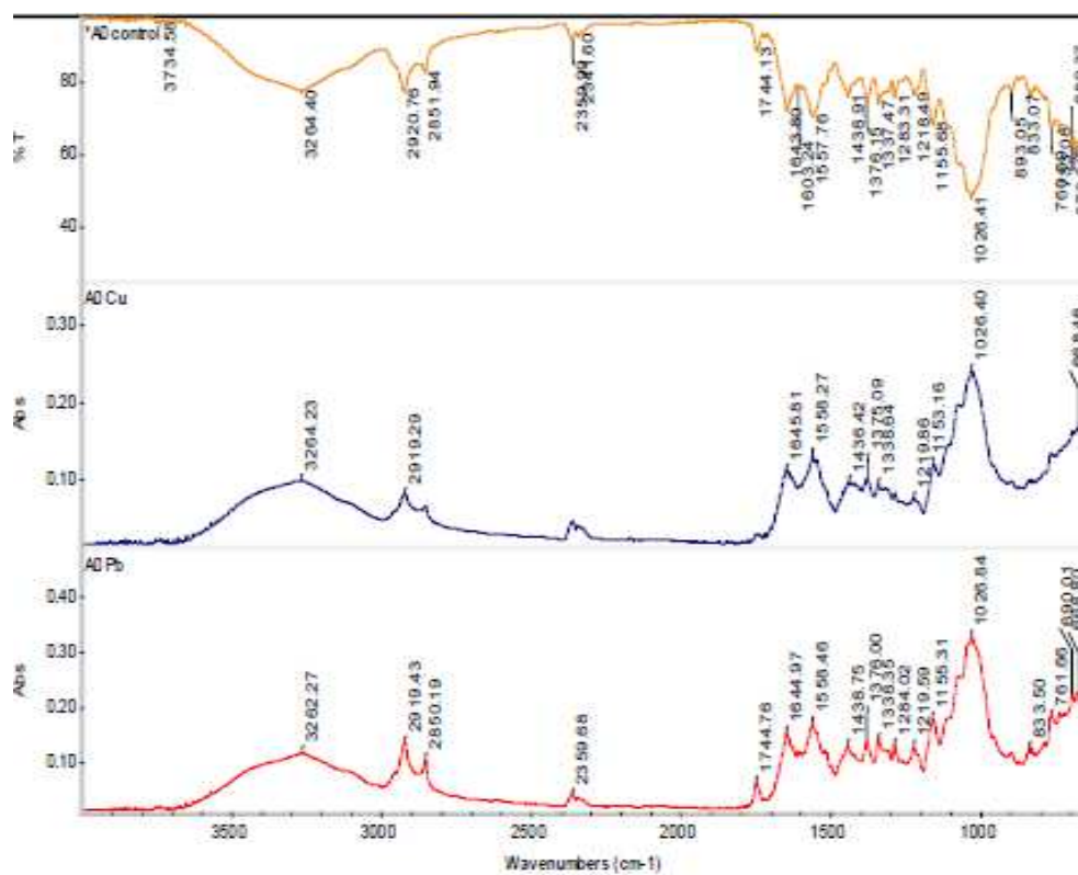
Fig. 11: FTIR spectra of dried unloaded (A0 control), lead(II)-loaded (A0 Pb), and copper(II)-loaded biomass of F. equiseti (A0 Cu).
