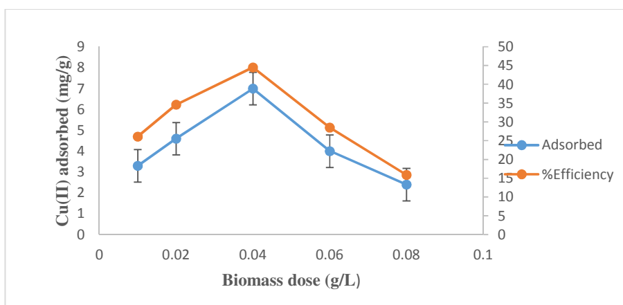
Figure 6: Copper (II) biosorption ( \text{mg g}^{-1} d.wt) and biosorption efficiency by Fusarium equiseti KR706303 at different biomass dose. Initial metal concentration ( C_i ): 50 \text{mg L}^{-1} ; suspension volume: 20 mL; temperature:
