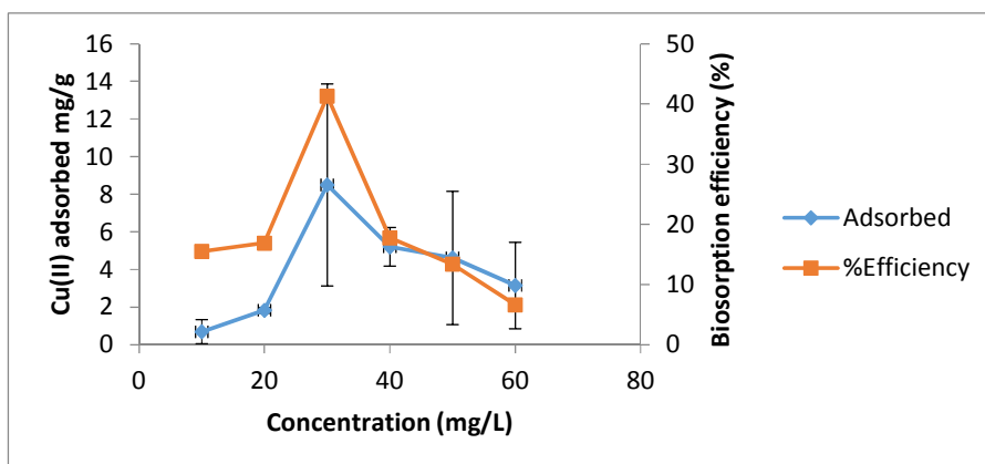
Figure 5: Copper (II) biosorption ( \text{mg g}^{-1} d.wt) and biosorption efficiency by Fusarium equiseti at different concentrations. Amount of dried biomass: 0.04 g; suspension volume: 20 mL; temperature: 30°C; pH: 9; agitation speed: 150 rpm. The data are the mean values of 3 replicates, and the bars indicate the standard deviation of the mean.
