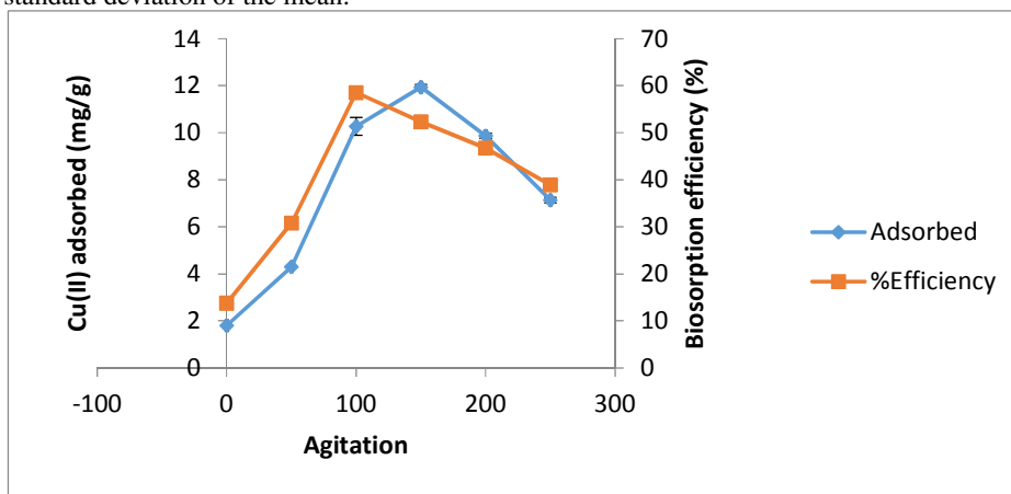
Figure 7: Copper (II) biosorption ( \text{mg g}^{-1} d.wt) and biosorption efficiency by Fusarium equiseti KR706303 at different agitation speed. Amount of dried biomass: 0.04 g; initial metal concentration ( C_i ): 50 \text{ mg L}^{-1} ; suspension volume: 20 mL; temperature: 30°C; pH: 9. The data are the mean values of 3 replicates, and the bars indicate the standard deviation of the mean
