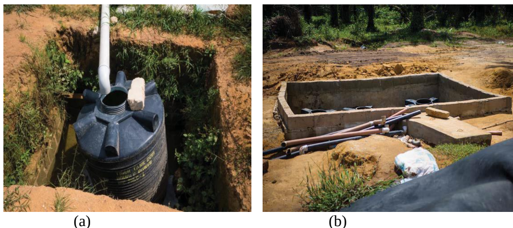
Figure 5: Poorly constructed and abandoned biocell drainage sumps. Source: Amnesty international.org
