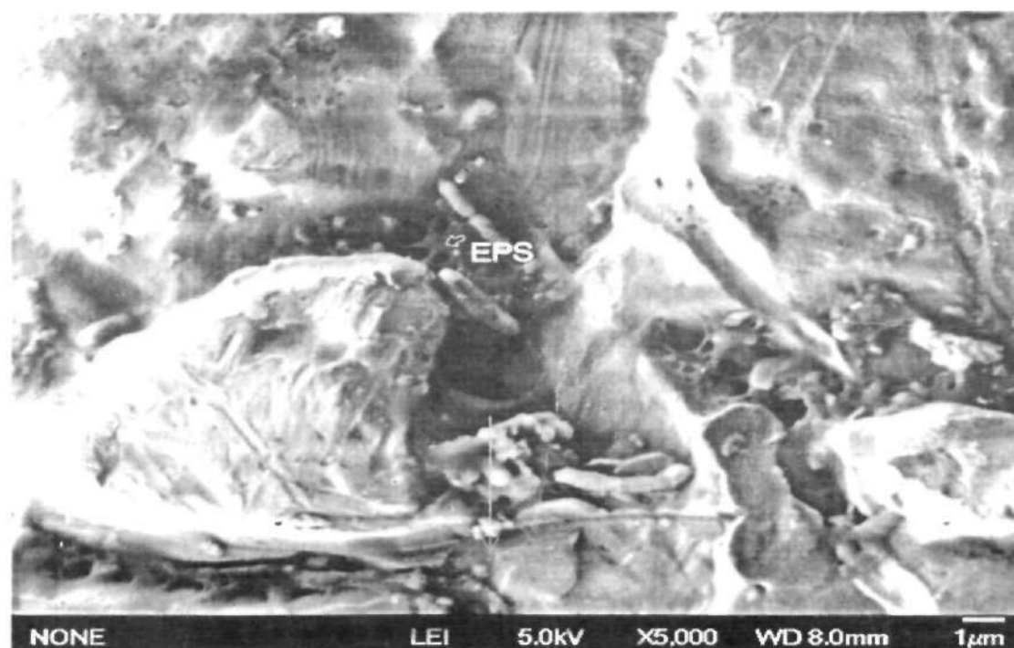
Figure 7: FESEM image of E. coli DH5a biofilm showing dehydrated EPS.
