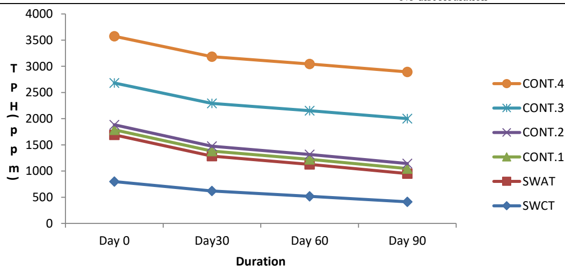
Figure 2: Total petroleum hydrocarbon (TPH) content of soils over 90 daysperiod of incubation
