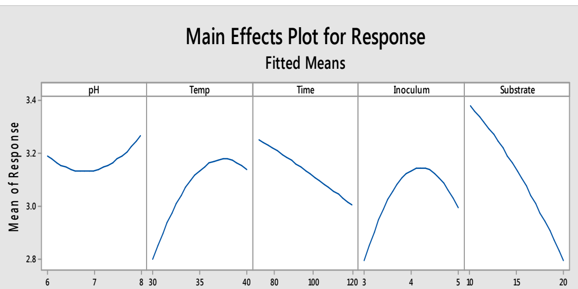
Fig 3: Main effect plot for carbohydrate (sugar) converted to ethanol
