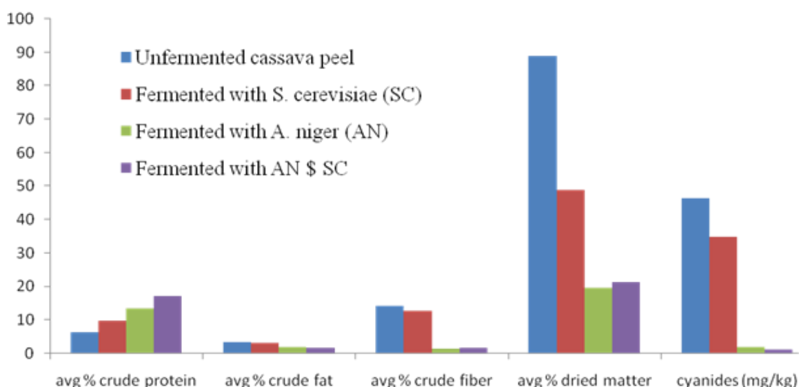
Figure 1a: Synergistic Effect of S. cerevisiae and A. niger on Cassava Peel Nutrient Composition after Fermentation
